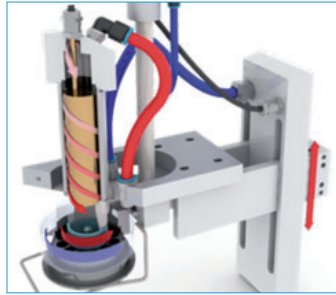
Sustainable energy savings with new state-of-the-art hot air cooling system
